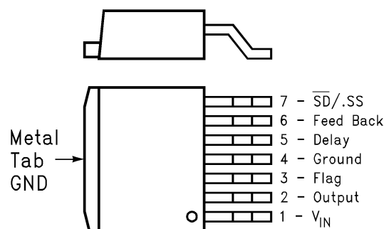
Figure 2. Surface Mount Package 7-Lead TO-263 (KTW) Package Number KTW0007B
