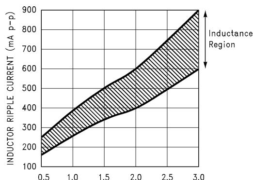
Figure 37. Peak-to-Peak Inductor Ripple Current vs Load Current
