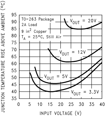
Circuit Data for Temperature Rise Curve TO-220 Package (NDZ)
